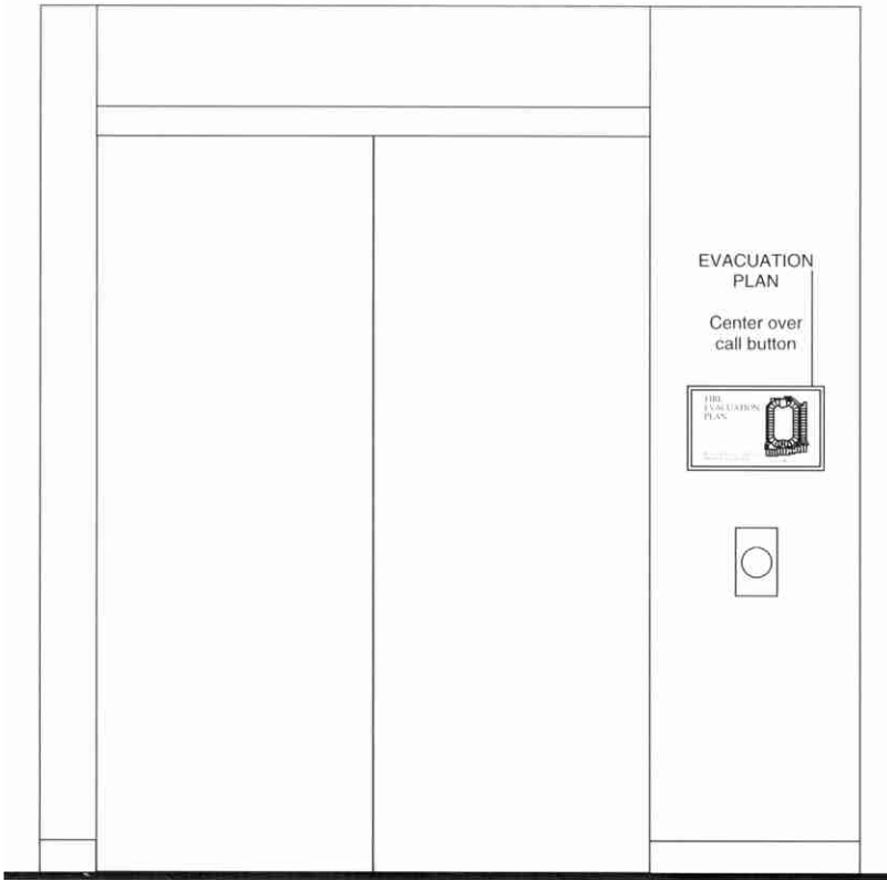
ELEVATOR EVACUATION ELEVATION (NOT TO SCALE)
