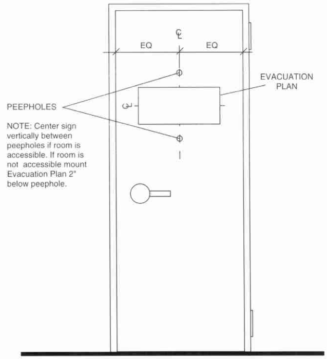
ROOM SIDE ELEVATION (NOT TO SCALE)
