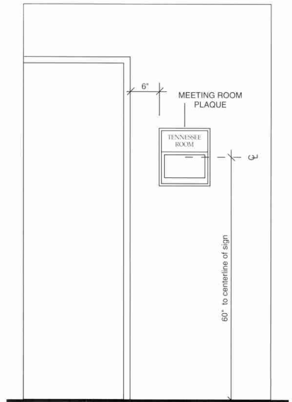
MEETING ROOM ELEVATION (NOT TO SCALE)
