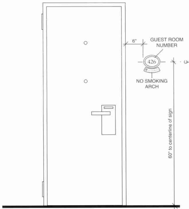
CORRIDOR SIDE ELEVATION (NOT TO SCALE)
